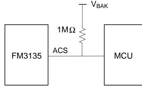
Figure 4. ACS Pin Requires Pullup
